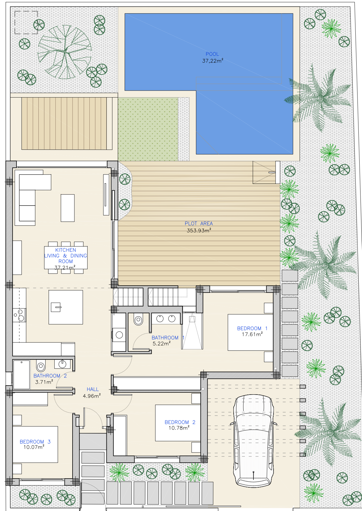
GROUND FLOOR
